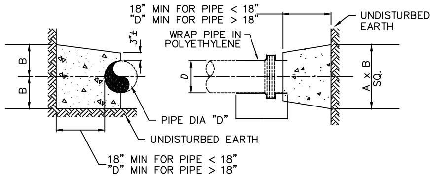
SECTION X-X BENDS & TEES
